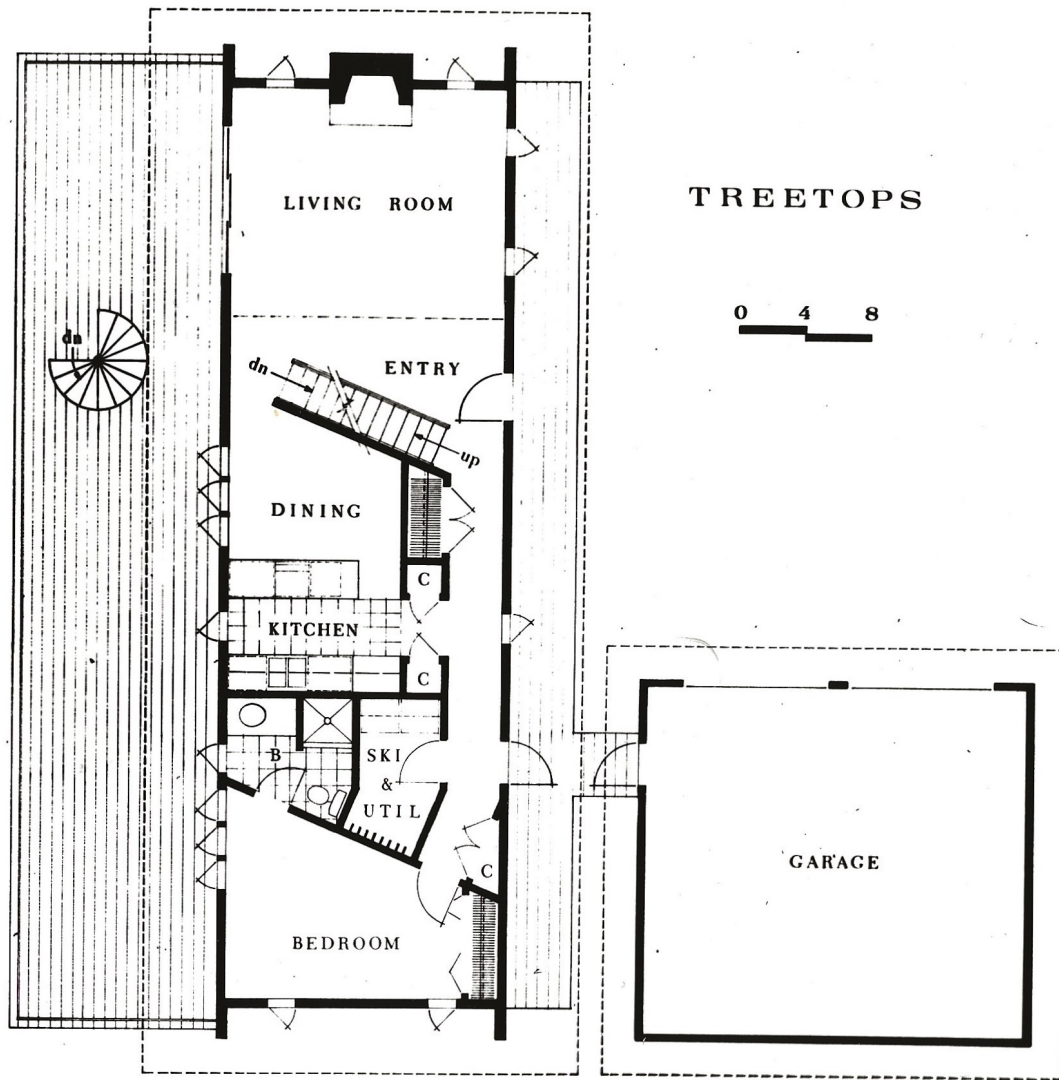
MAIN FLOOR
